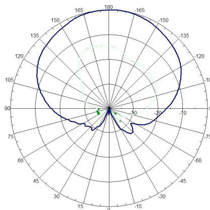
Slant port, horizontal
