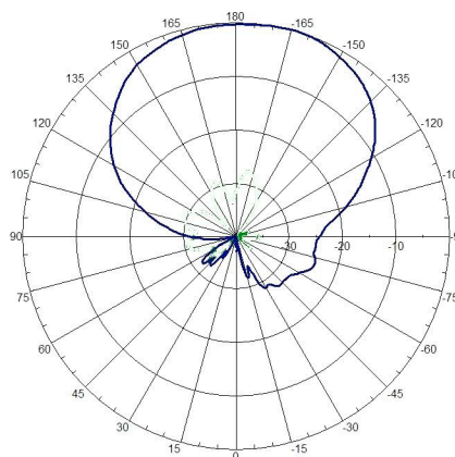
Horizontal polarization port, horizontal
