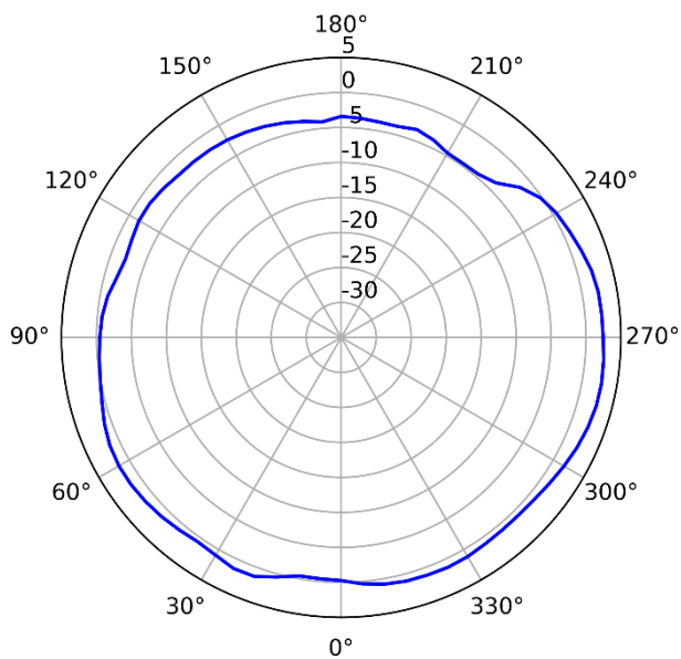
2.4GHz (Horizontal)
